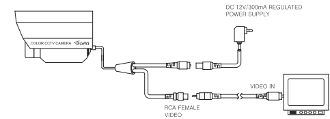
RCA CONNECTION(STANDARD)
