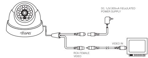
RCA CONNECTION(STANDARD)
