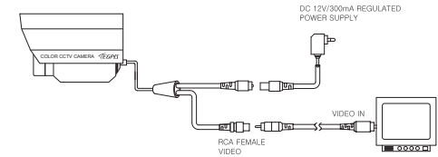
RCA CONNECTION(STANDARD)
