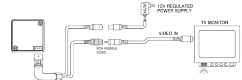
RCA CONNECTION(STANDARD)
