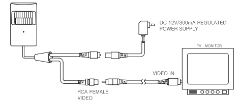
RCA CONNECTION(STANDARD)
