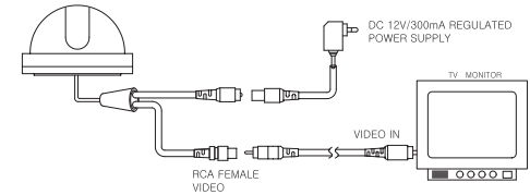
RCA CONNECTION(STANDARD)
