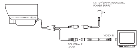
RCA CONNECTION(STANDARD)
